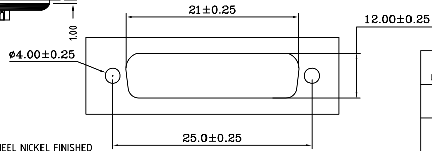
9P Bore hole drawing REF
