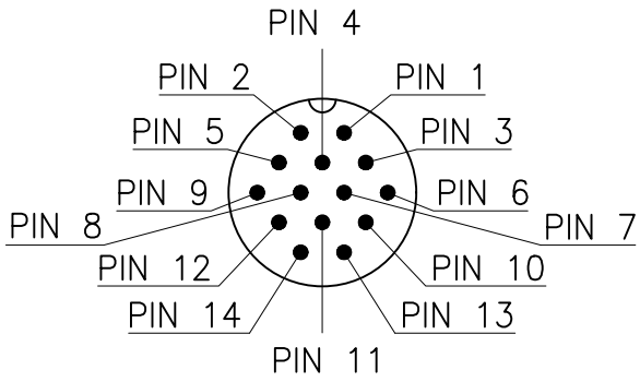
VIEW A
