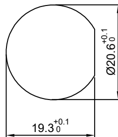
Dimensions of panel openings
