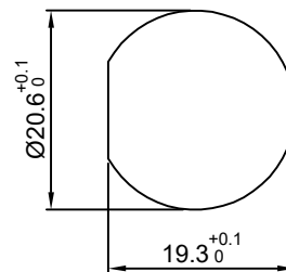
Dimensions of panel openings
