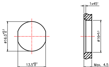
Panel Cut-out for M16x1.5
